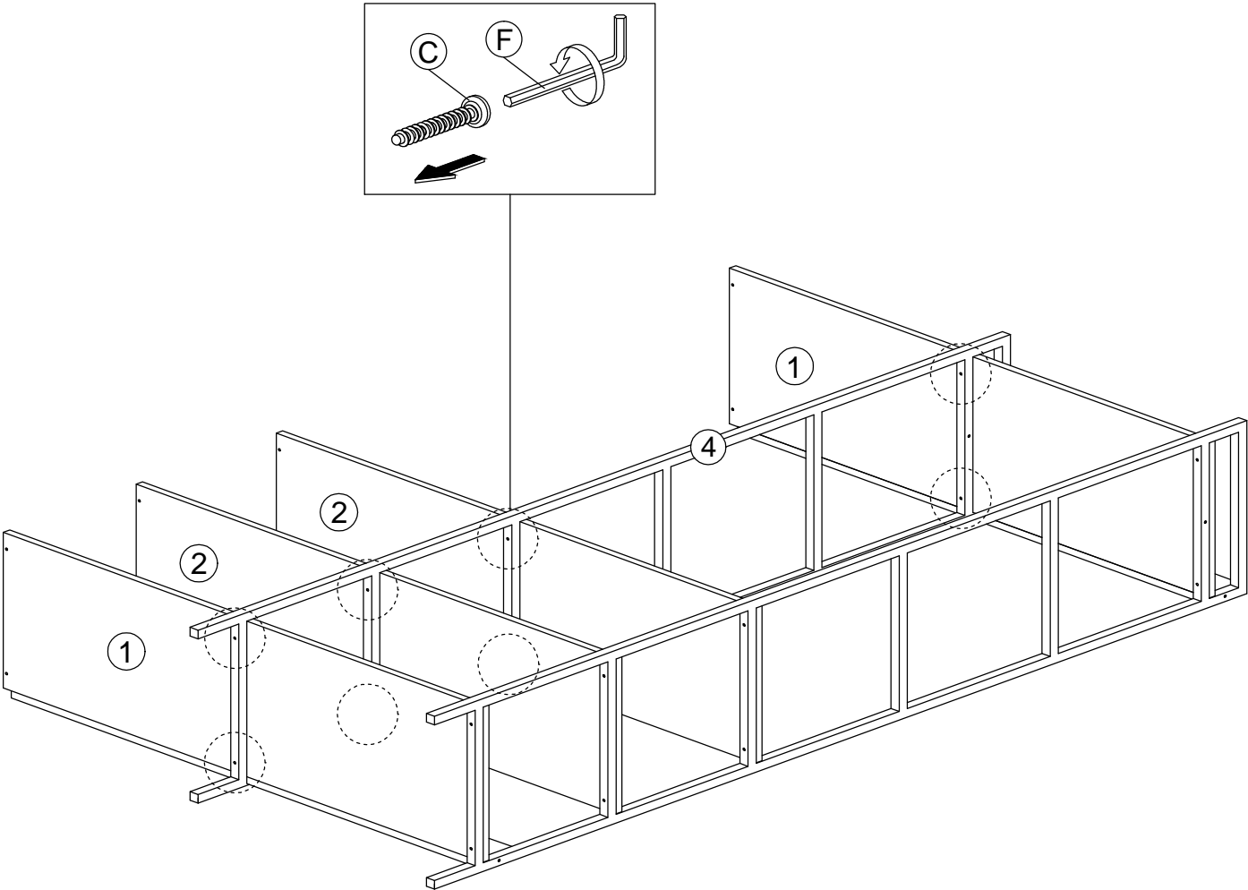
BOTTOM VIEW
