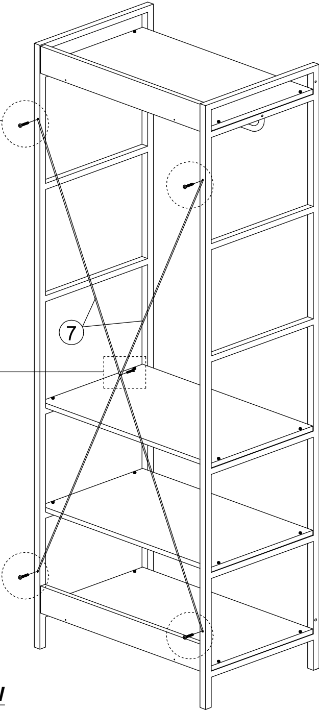
BACK VIEW
